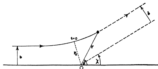
FIG. 1. Classical trajectory.
